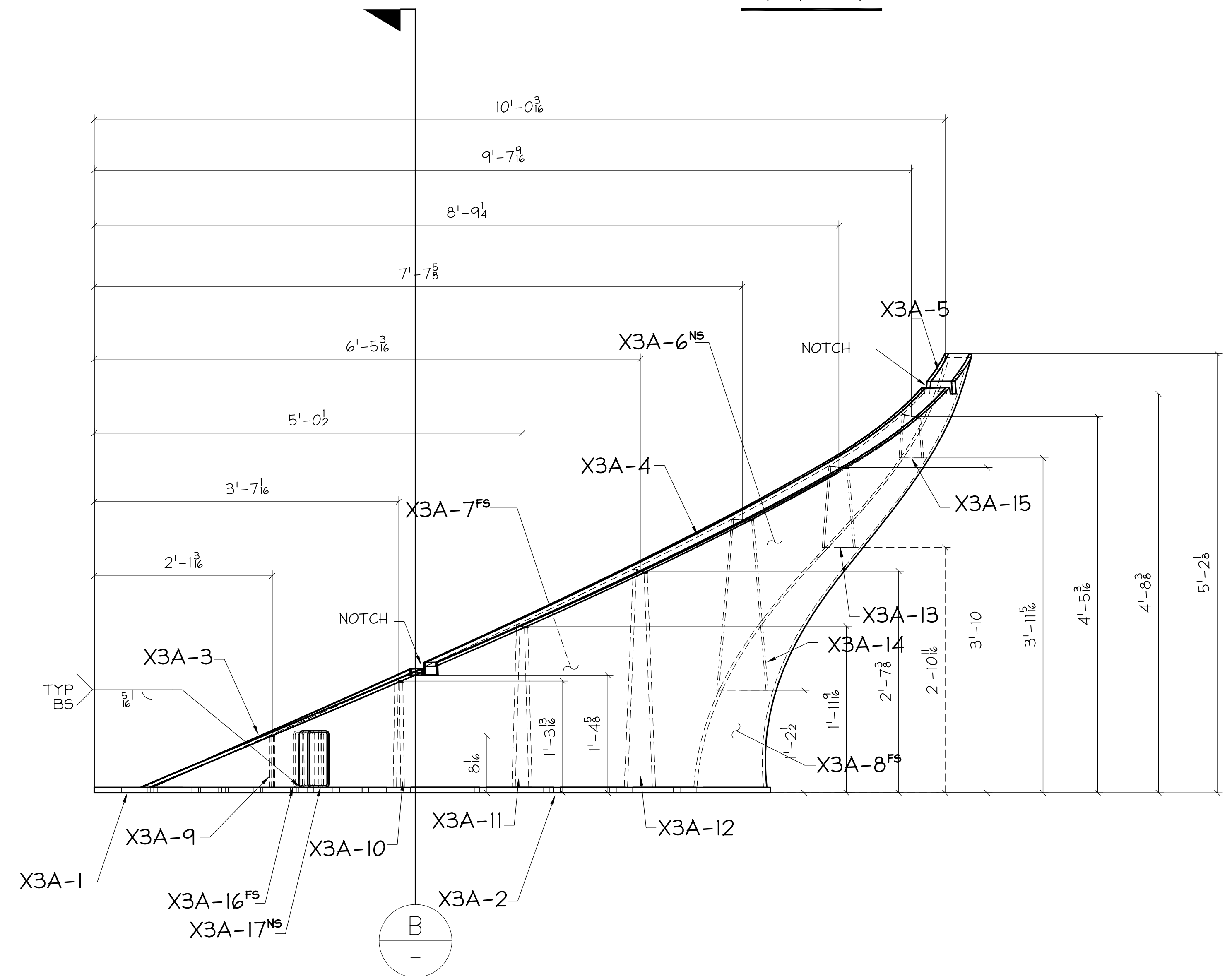
SECTION A STAIR PEDESTAL ELEVATION VIEW
