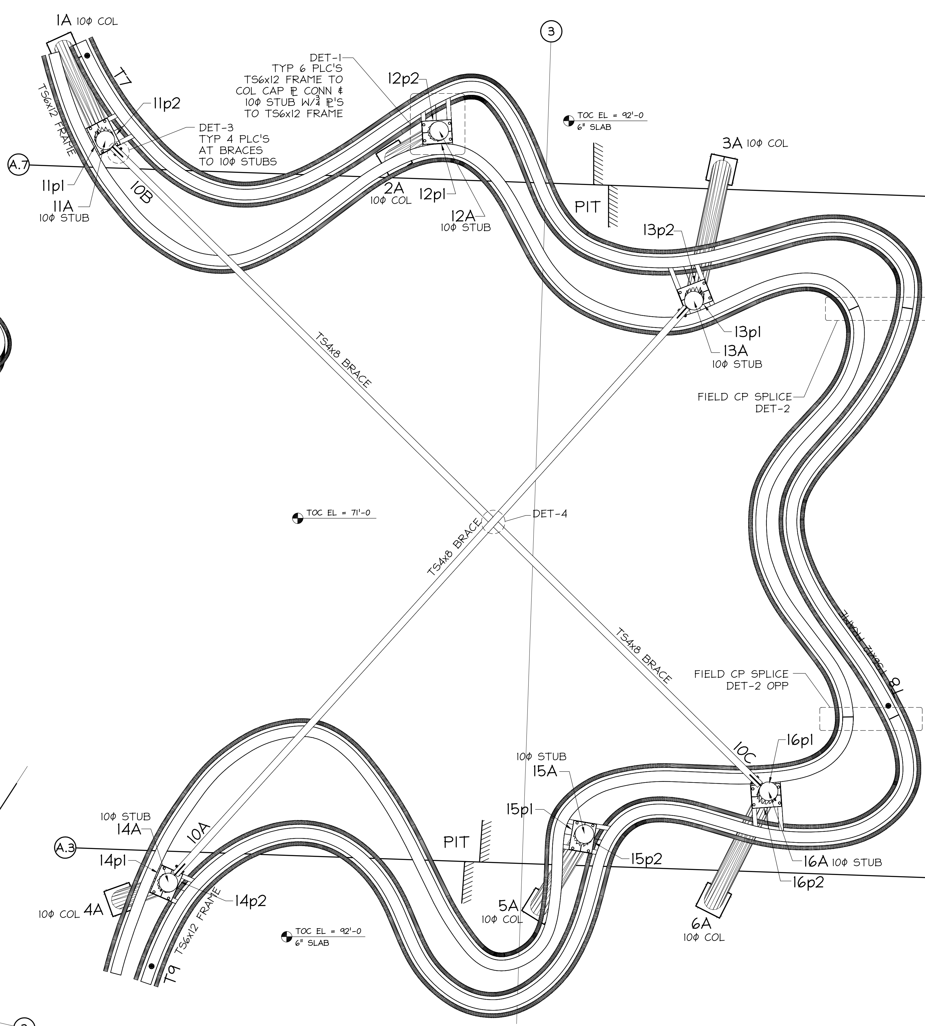
PLAN VIEW ~ CHAIN LINK WALL
